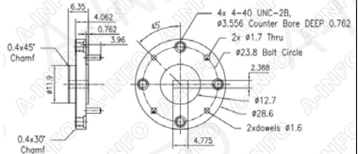
FUGP500 (equivalent to UG-383/U modified)
