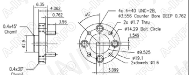
FUGP740 (equivalent to UG-387/U)
