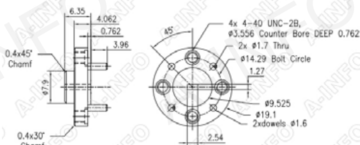
FUGP900 (equivalent to UG-387/U modified)
